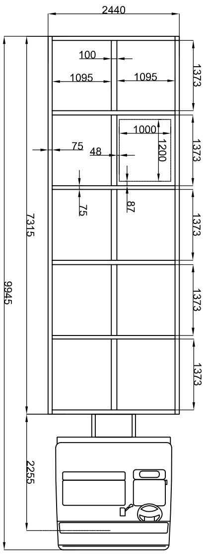
PLAN
